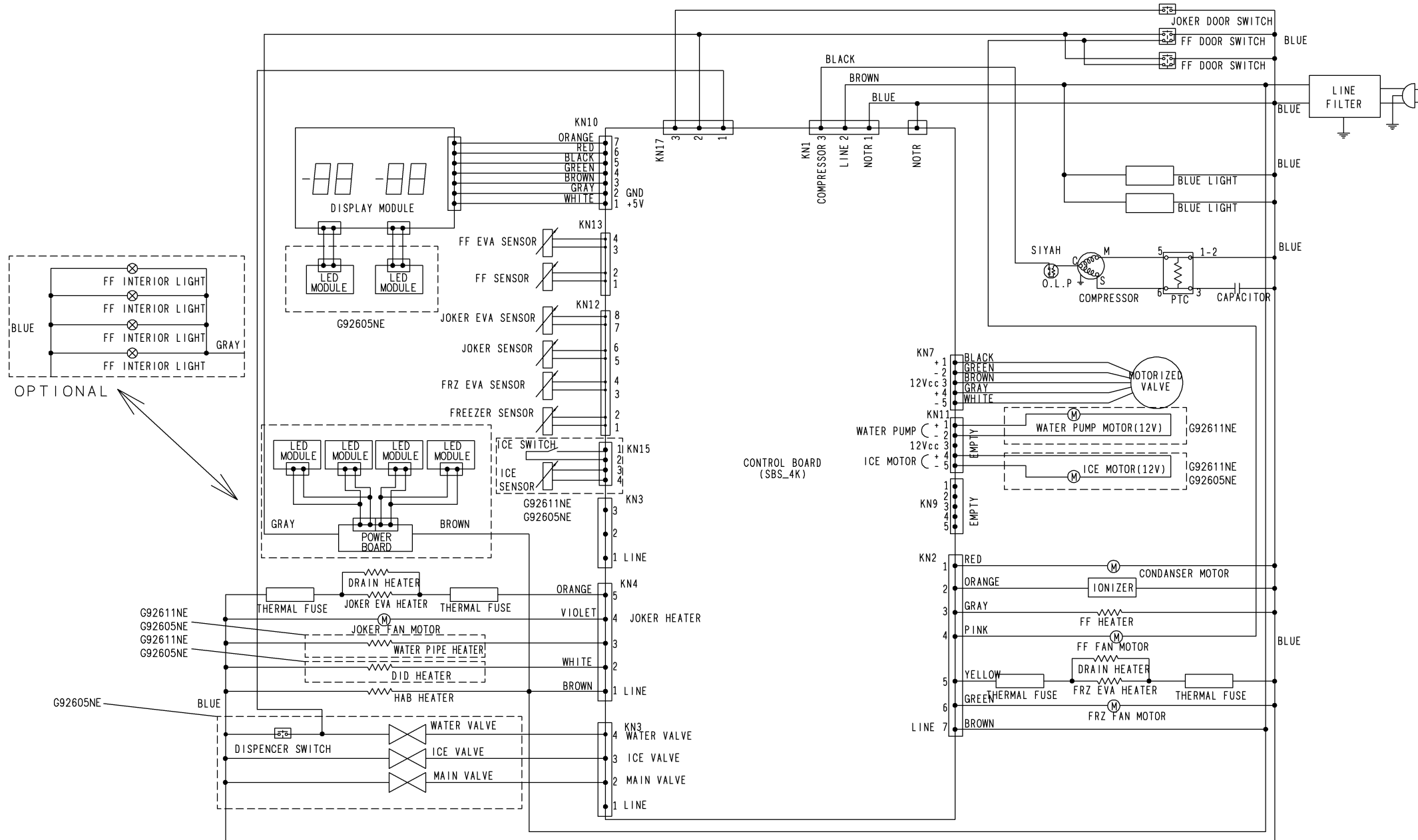
CIRCUIT DIAGRAM V1_G92610NE V2_G92611NE V3_G92605NE
