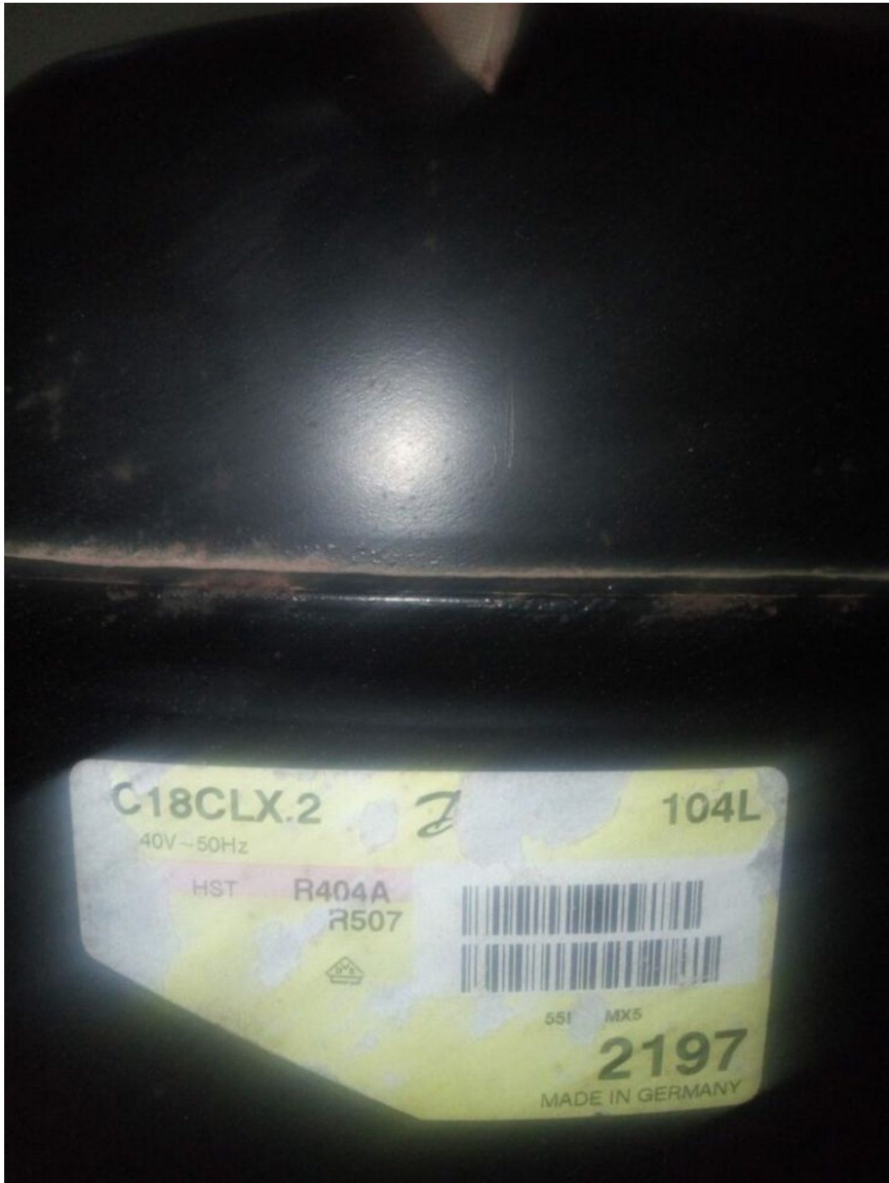
Mbsm.pro, compressor, Secop, SC18CLX.2, 104L2197, Danfoss R404A, R507, 3/4 hp, 1bp
