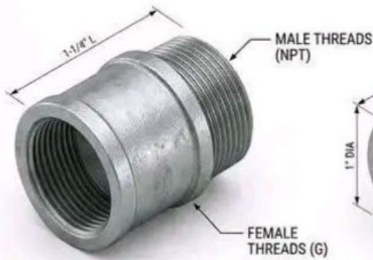
(1) COUPLING
