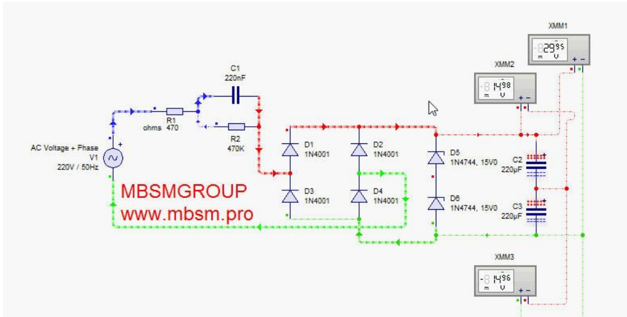
Mbsm.pro , Schema Electronique Alimentation 220v Ac 15/30 DC
