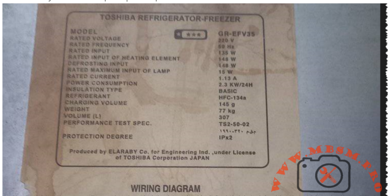
Mbsm.pro, TOSHIBA, REFRIGERATOR, FREEZER, GR-EFV35, 12 feet, 3 D00R, 307 L, compressor, 1/5 hp, 140 w, lbp, r134a, 145 g
