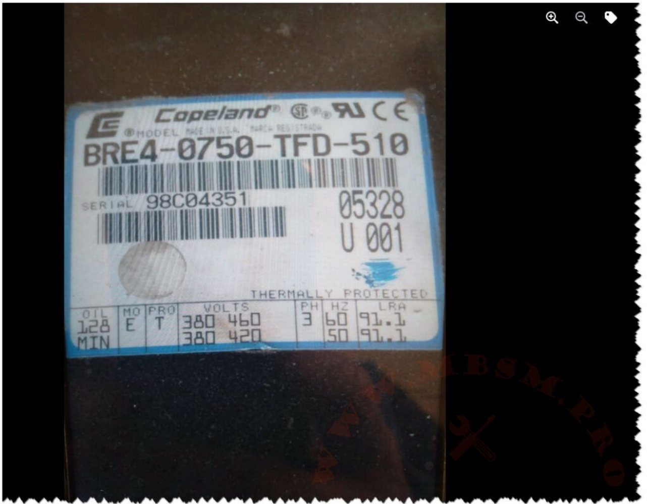
Mbsm.pro, compressor, BRE4-0750-TFD-510, Copeland, 7.5 HP, 460V, 3 PH, R22, R134A, R407C, Scroll Compressor, Copeland Compressor
