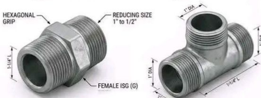
(3) REDUCER HEX NIPPLE
