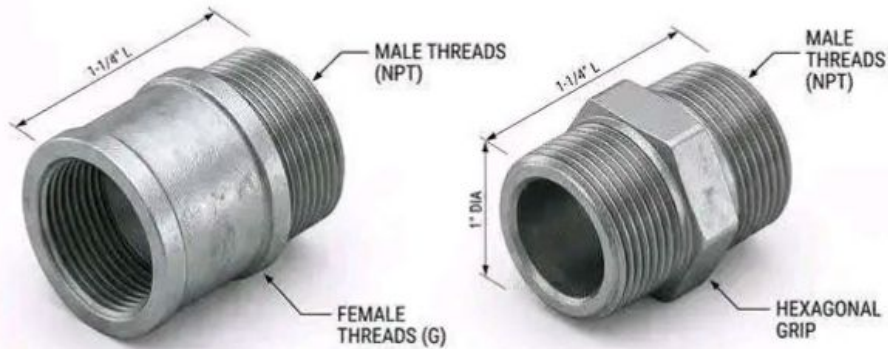
(1) COUPLING
