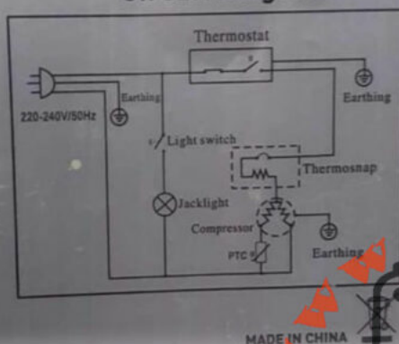
Circuit Diagram
